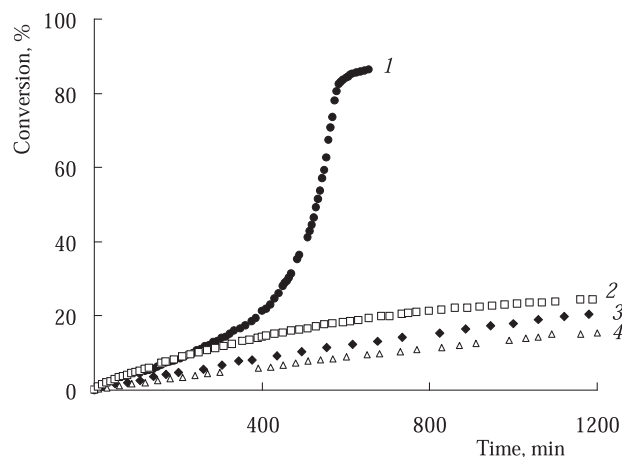
Figure 7. Conversion vs. MMA polymerization time at 60°C in the presence of BP (1), BP and porphyrins 6 (2), 5 (3) and 4 (4). [\text{BP}] = [\text{4}] = [\text{5}] = [\text{6}] = 1.0 \text{ mmol/l} .
