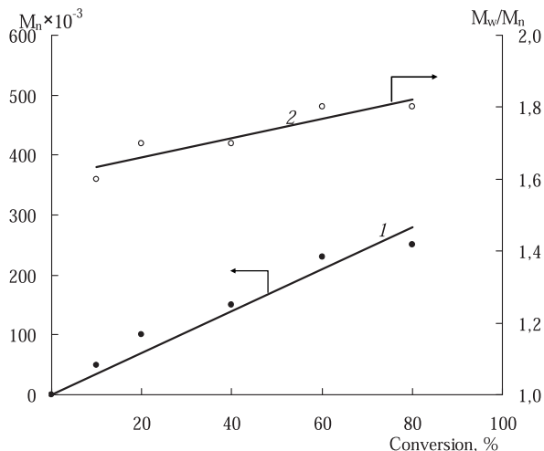
Figure 6. M_n (1) and M_w/M_n (2) of polystyrene obtained in the presence of AIBN and porphyrin 6 at 100°C vs. monomer conversion. [\text{AIBN}] = [\text{6}] = 1.0 \text{ mmol/l} .
