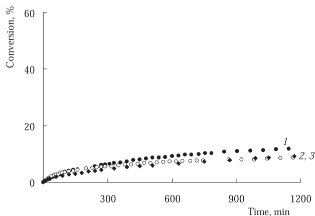
Figure 12. Conversion vs. MMA polymerization time at 60°C in the presence of BP and porphyrins 7 (3), 8 (1) and 9 (2). [BP] = [7] = [8] = [9] = 1.0 mmol/l.
