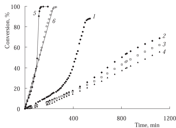
Figure 3. Conversion vs. MMA polymerization time at 60°C ( 1-4 ) and 80°C ( 5, 6 ) in the presence of AIBN ( 1, 5 ), AIBN and porphyrin 4 ( 2-4, 6 ). [AIBN] = 1.0 mmol/l; [ 4 ] = 0.5 ( 2 ), 1.0 ( 3 , 6 ) and 3.0 ( 4 ) mmol/l.
